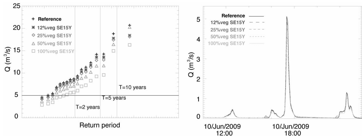
Figure 2. Results of the SWMM simulations for Châtillon basin by using the different green roofing scenarios: the statistical distribution of annual peak discharge is represented on the left (5 m 3 /s threshold is indicated) and the storm event of June 2009 is represented on the right.
