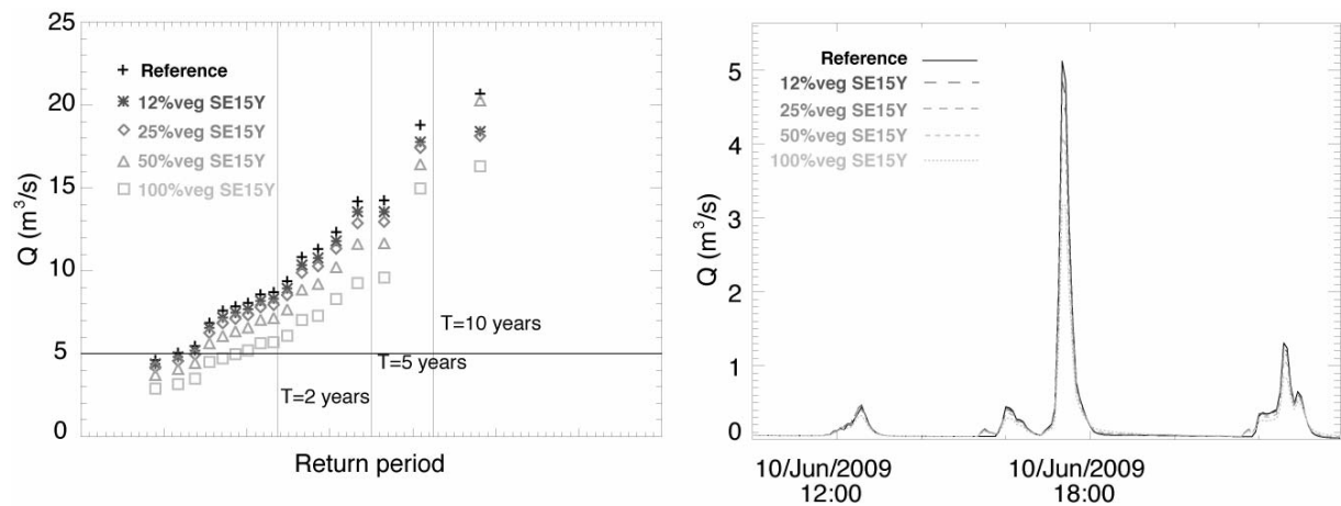
Figure 2. Results of the SWMM simulations for Châtillon basin by using the different green roofing scenarios: the statistical distribution of annual peak discharge is represented on the left (5 m 3 /s threshold is indicated) and the storm event of June 2009 is represented on the right.
