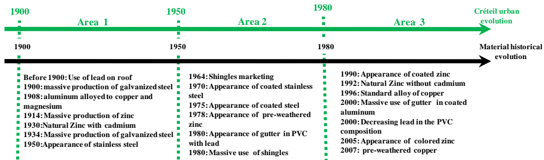
Figure 4: The historical evolution of roofing material emitting of zinc
