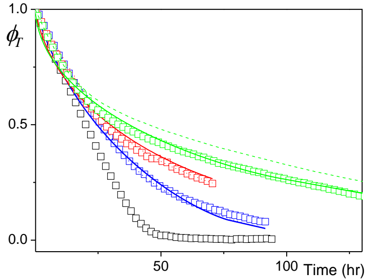
FIG. 4. Total water saturation (ratio of the total mass of water to the initial mass of water ) as a function of time during the drying of a porous medium. Initially filled with: (black) pure water, (blue) 5% colloidal particles in water, (red) 10%, (green) 15%. The square symbols correspond to the experimental data. The dotted lines correspond to the modelling approach based on the measure of the compacted front thickness, and the continuous lines to the full modelling approach.
