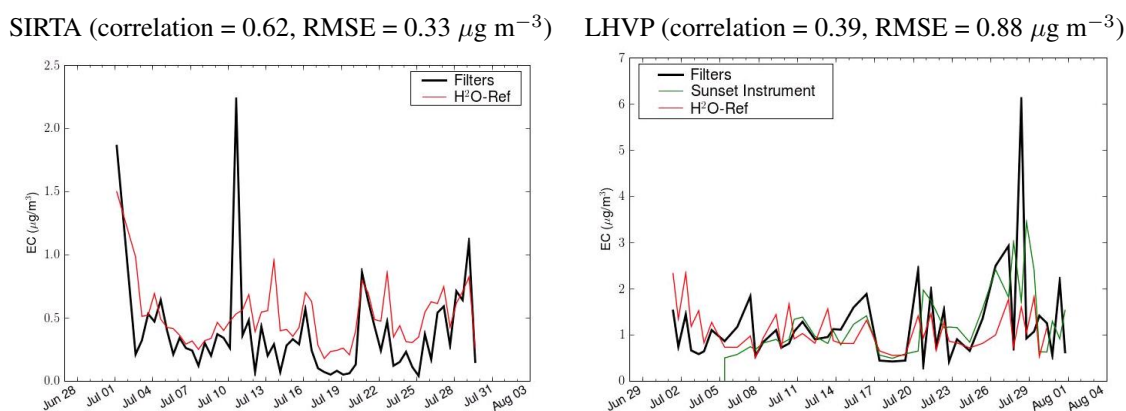
Fig. 4. 12 h averaged concentrations of EC modeled with “H 2 O-Ref” and measured with filters at the SIRTA site (left) and with both filters and Sunset filed instrument at the LHVP (right) site (correlations and RMSE are between the model and the filter measurements).
