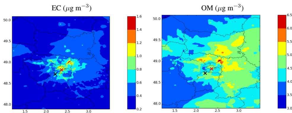
Fig. 3. Simulated concentrations in \mu\text{g m}^{-3} of EC (left) and OM (right) for July 2009. The red and black crosses correspond to the LHVP and SIRTA sites, respectively.
