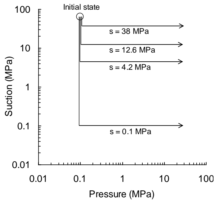
Figure 4. Stress paths followed in the suction controlled oedometer tests
