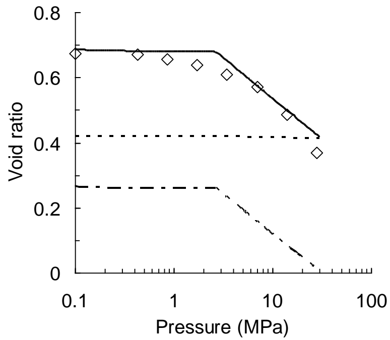
Figure 6. Void ratio changes upon mechanical loading at constant suction
