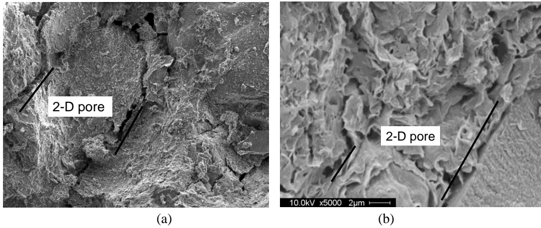
Figure 11 2-D pores with diameter of 50μm (a) and 1μm (b)
