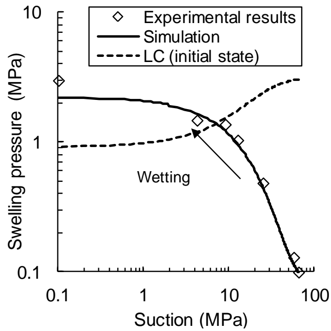
Figure 8. Changes of swelling pressure during suction decrease under constant volume condition
