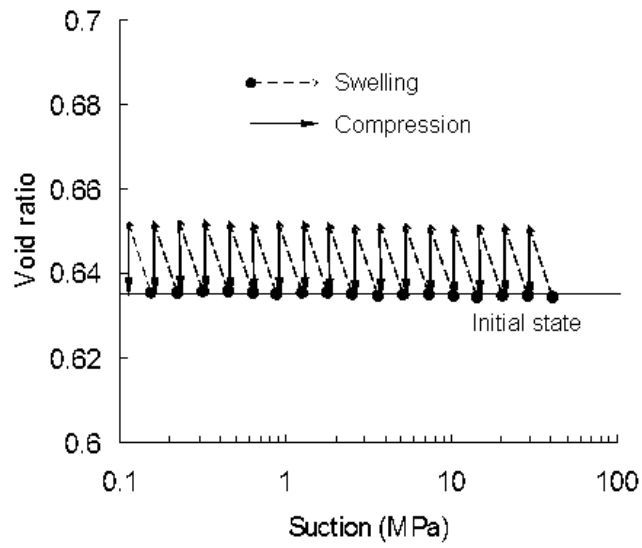
Figure 7. Stress path followed during the swelling pressure simulation
