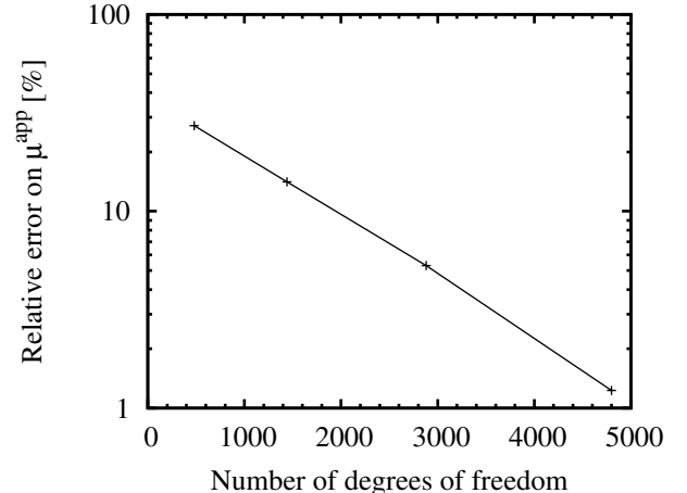
Figure 7: Relative error on \mu^{\text{app}} as a function of the number of degrees of freedom of the EIM-G, in semi-log scale. Convergence seems to be exponential.
