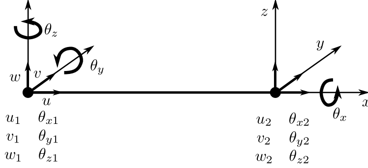
Figure 9: Displacement finite element
