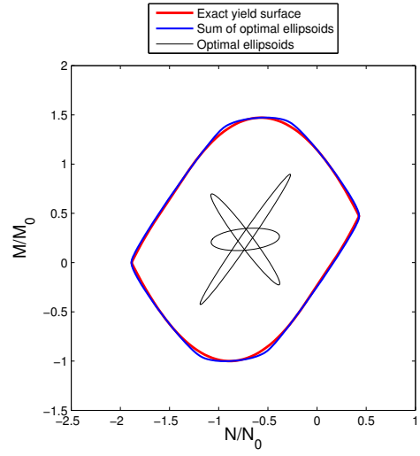
(b) n_{ell} = 3
