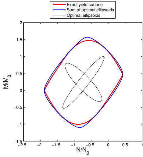
(a) n_{ell} = 2
