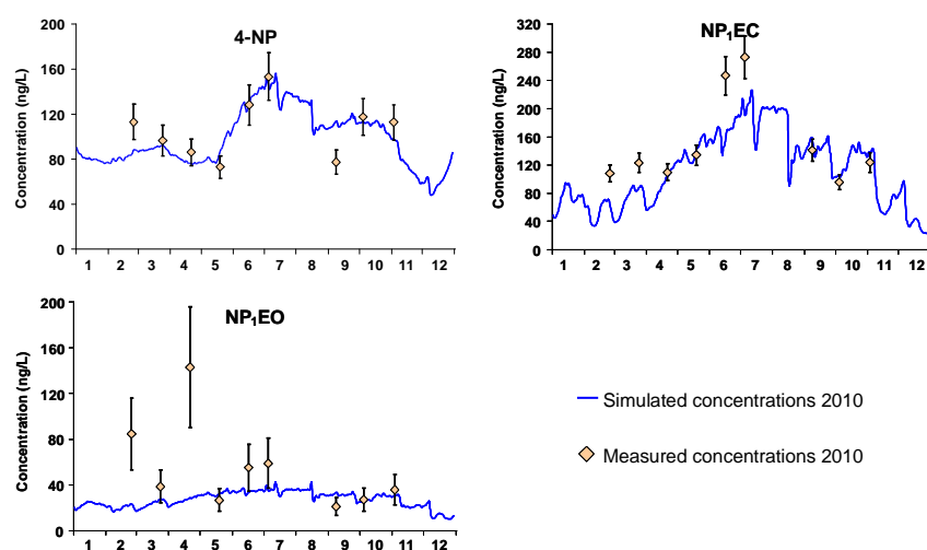
15 Fig. 5 Simulated concentrations of 4 NP, NP 1 EC and NP 1 EO at Meulan using the Prose model (September 16 parameter set) versus measured concentrations 17 18
