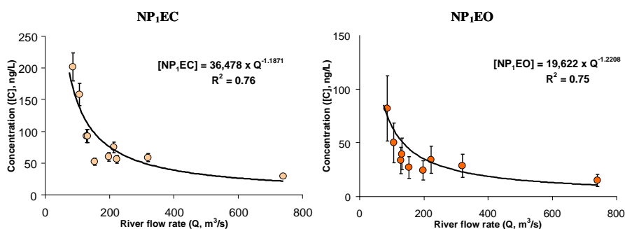
4 Fig. 3 Relationships between NP 1 EC and NP 1 EO concentrations and Seine River flow at Bougival 5 6
