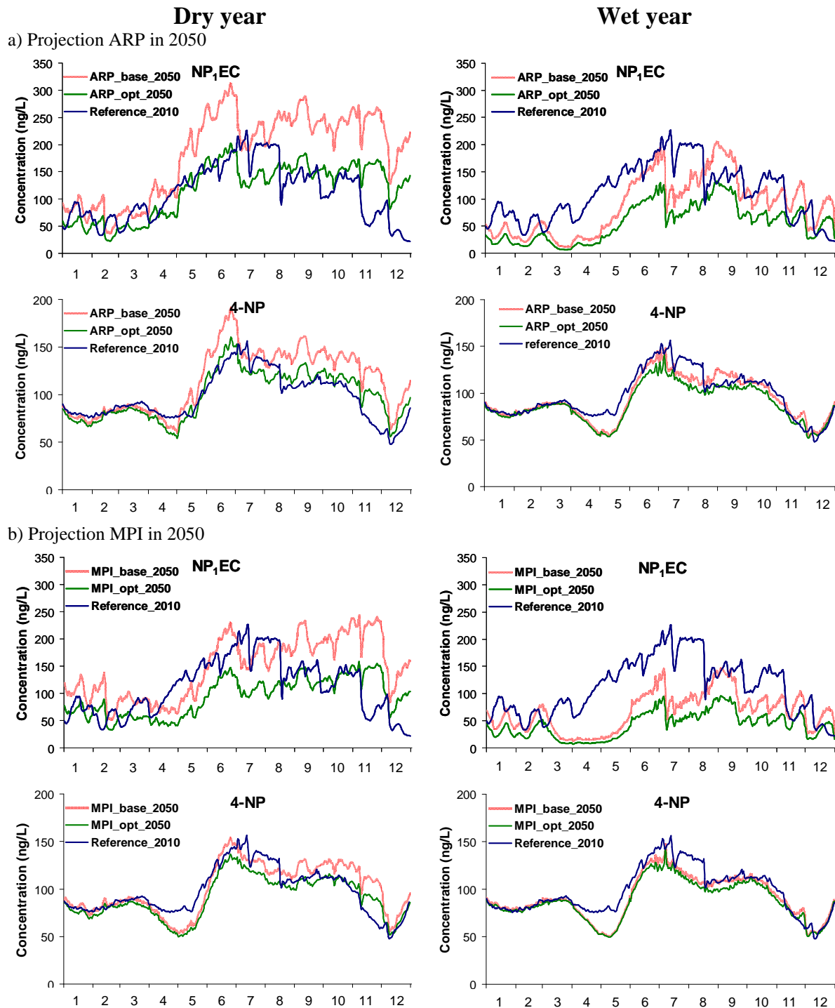
1 Fig. 6 Forecasted concentrations of 4 NP and NP 1 EC for one dry and wet year in the decade 2045 - 2055
