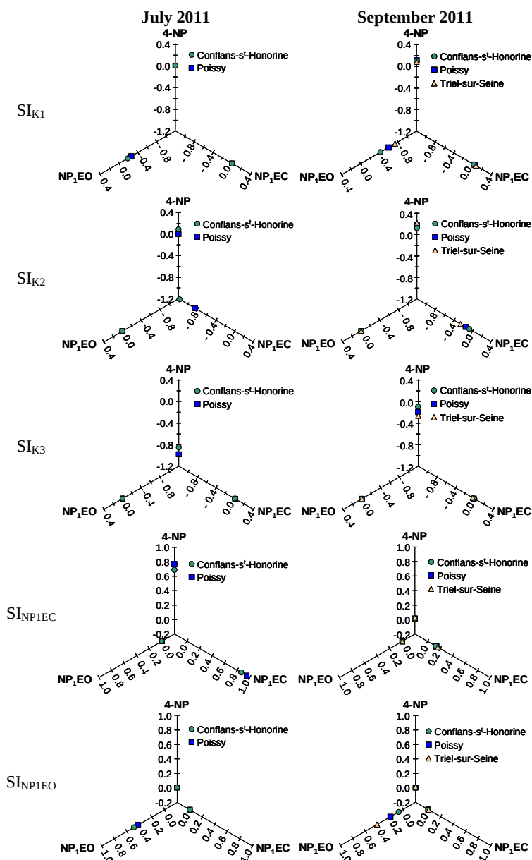
Fig. 6 Sensitivity indexes of simulated concentrations of 4-NP, NP 1 EO and NP 1 EC at Conflans-st-Honorine, Poissy and Triel-sur-Seine towards attenuation rate constants and precursor inputs
