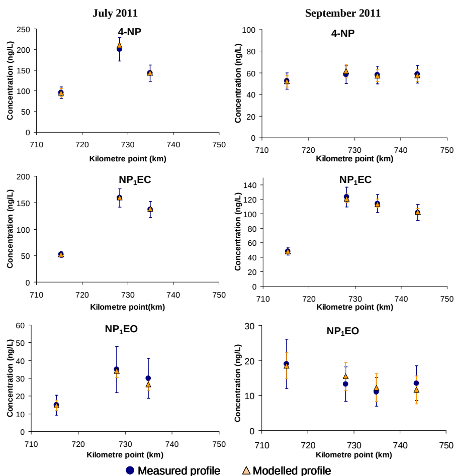
Fig. 5 Modelled (optimised rate constants) and actual profiles of 4-NP, NP 1 EC and NP 1 EO concentrations in the Seine River. The points exhibited are Maisons-Laffite (715.4 km), Conflans-st-Honorine (728.2 km), Poissy (734.9 km) and Triel-sur-Seine (743.6 km). The y error bars represented on the actual profile indicate the total variabilities linked to in-situ sampling while they represent the uncertainties attached to boundary conditions on modelled profile
