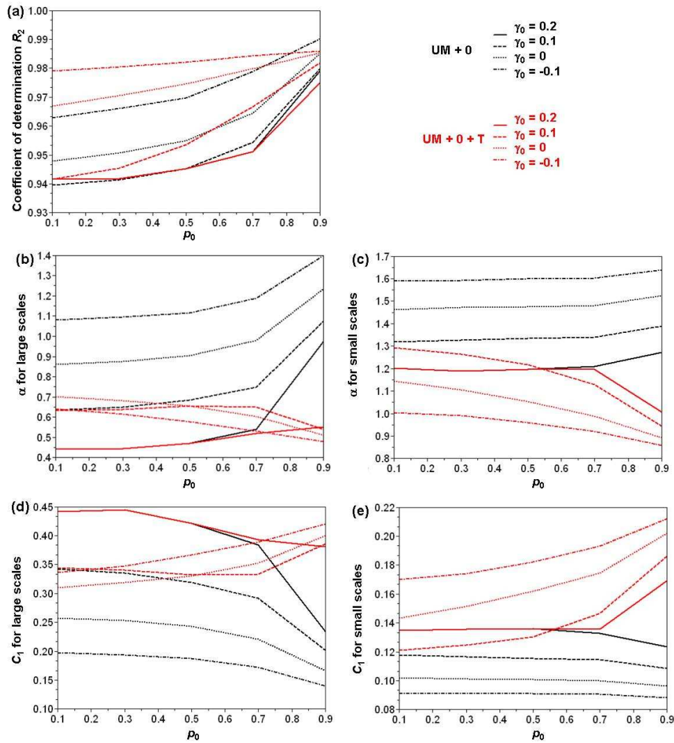
Fig. 7. Analysis of the sensitivity to \gamma_0 and \rho_0 : coefficient of determination R^2 of the linear regression in the TM analysis for q = 2 (a) , \alpha and C_1 for large and small scales (b, c, d, e).
