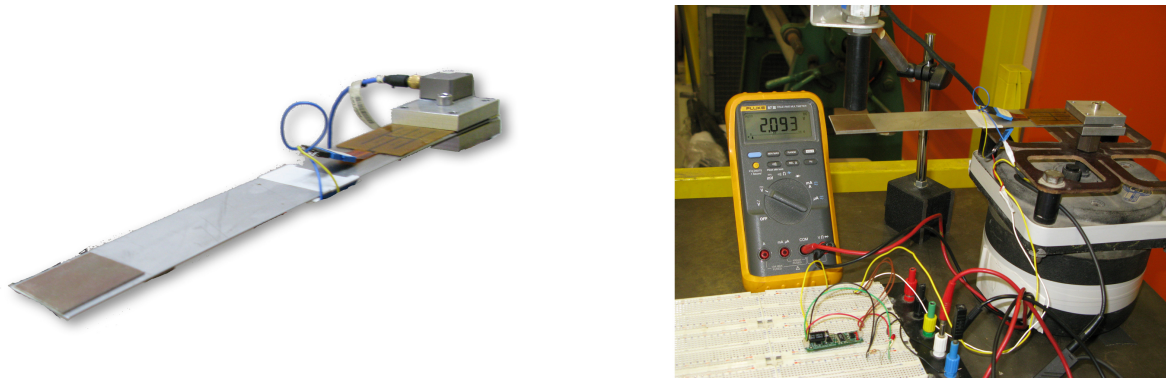
Figure 10. Piezoelectric harvester designed for traffic-induced vibrations (left), and view of the test set-up (right).
