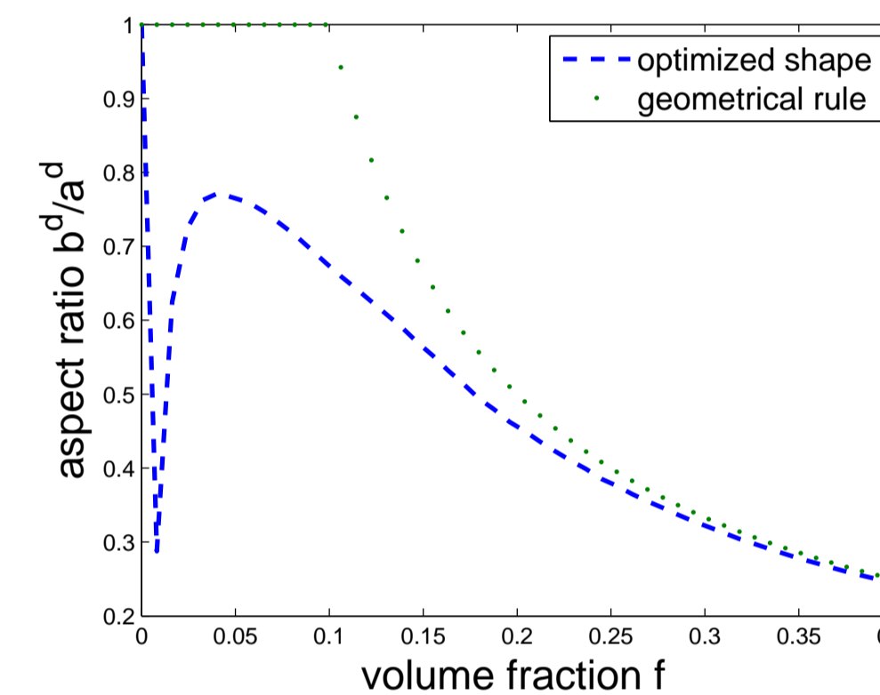
Fig. 3: Two possibilities for the evolution of the aspect ratio of the atmosphere
