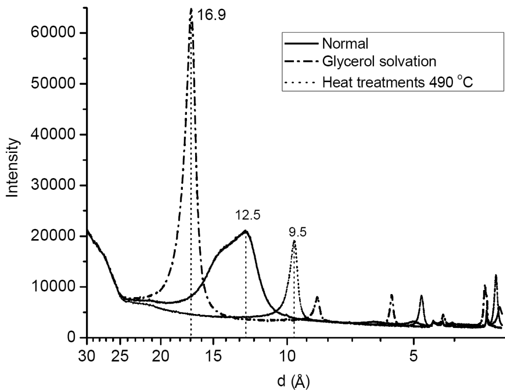
Figure 2. X-Ray curves of the MX80 bentonite
