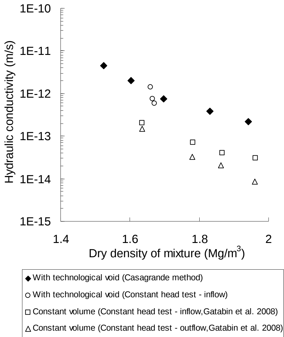
Figure 15. Hydraulic conductivity versus dry density of mixture
