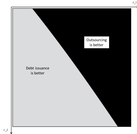
Fig. 3 Decision areas in Nash equilibrium
