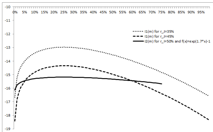
Fig. 1 Value functions \hat{I}^1 and \hat{I}^2 as functions of \hat{m}
