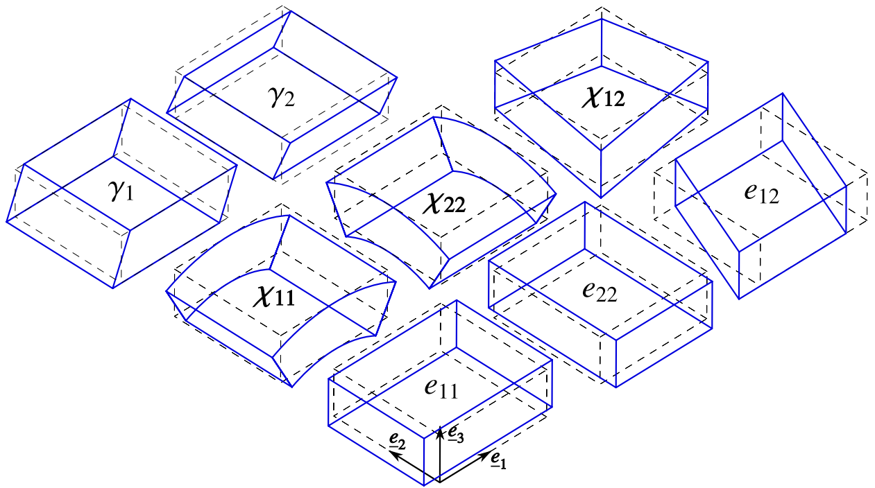
Figure 3: Reissner-Mindlin generalized strains
