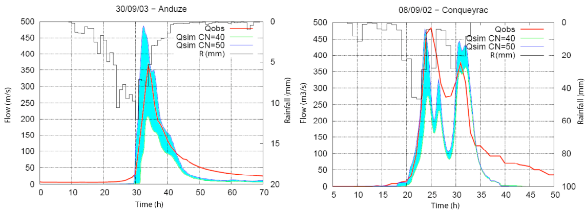
Fig. 4. Comparison between simulated and measured hydrographs – validation.
