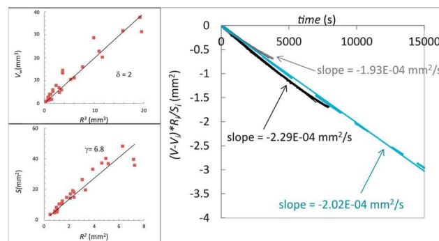
Fig. 9 Left: geometry of the coated droplet: initial volume (top) and initial surface area (bottom) as a function of initial radius of curvature; right: temporal evolution of the normalized volume ( (V - V_i) R_i / S_i ) for three coated drops of different initial volumes ( V_i = 7 mm 3 , 27 mm 3 and 67 mm 3 ).
