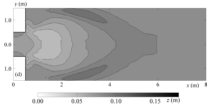
Figure 12. Computed bed topography for Case 1: Fine-mesh results by (a) WUH and (b) MISS. Coarse-mesh results by (c) EDF2 and (d) UNA2
