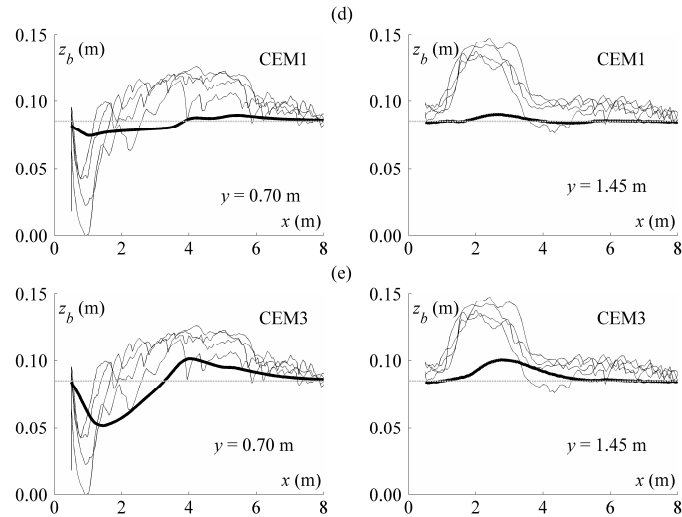
Figure 13. Influence of the sediment transport formula and closure parameters analysed from the results by Cea et al. (a-b-c) and Paquier and Le Coz (d-e): (a) \tau_c^* by Parker and q_s by Meyer-Peter and Müller, (b) \tau_c^* by Parker and q_s by Van Rijn, (c) \tau_c^* by Shields and q_s by Van Rijn, (d) \tau_c^* = 0.047 (Shields) and q_s by Meyer-Peter and Müller, (e) \tau_c^* = 0.15 and q_s by Meyer-Peter and Müller. The light grey lines refer to experimental results; the thicker line to the numerical results.
