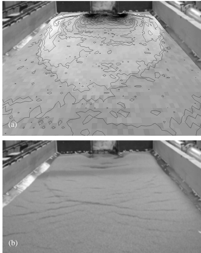
Figure 8. Final bed topography for Case 1: (a) perspective view from downstream, reconstructed from the measured bed profiles and (b) photograph taken after removing the water at the end of the experiment.
