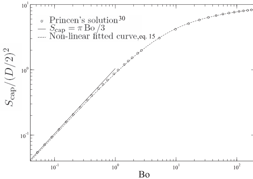
FIG. 7. S_{\text{cap}}/(D/2)^2 versus \text{Bo} : circle points are determined according to Princen's model 30 and dashed line is the fit corresponding to Eq. (15). The solid line is the asymptotic behavior at small Bond number according to Howell's model. 20
