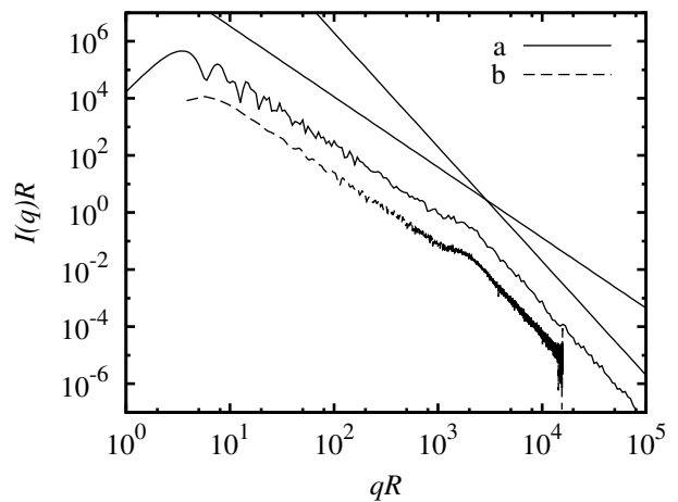
FIG. 19. Scattered intensity pattern of the Apollonian packing shown in figure 18, computed with the method proposed in this paper (a), and with the approximate formula (33) (b). The two curves are in excellent agreement, and match perfectly without rescaling; for the sake of readability, curve (b) has been translated vertically. The two straight lines represent the expected fractal ( I(q) \propto q^{-2.47} , low q ), and Porod ( I(q) \propto q^{-4} , high q ) regimes. In order to allow for the direct comparison of the two methods, both q and I(q) have been made dimensionless through multiplication by the external radius R of the packing; furthermore, \Delta \rho = 10^{10} R^{-2} .
