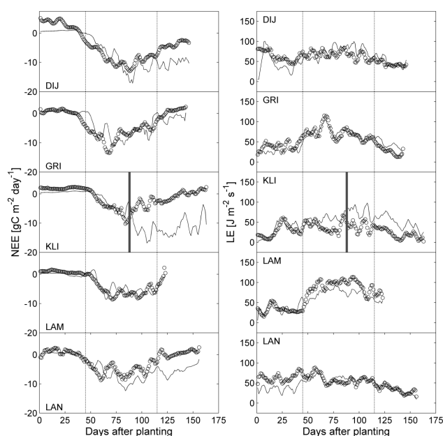
Fig. 4. Evolution of 5-days smoothed NEE (left) and LE (right) during the growing period at the five maize sites. Circle symbols indicate eddy covariance observed values and blue line indicates values simulated by ORCHIDEE-STICS. The fluxes are smoothed over consecutive 5 days. The first vertical dashed line x = 45 is defined as the end of the early crop growth period, and x = 115 is defined as the start of the late crop growth period. Between the two lines, it is defined as the middle crop growth period. The solid bold line at KLI subplot indicates the hail storm event on x = 88 .
