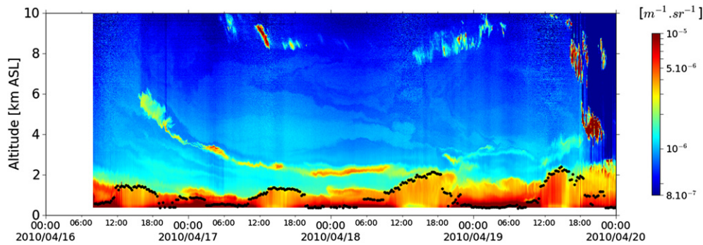
Fig. 1. Time series of the vertical profile of linearly polarized Lidar attenuated backscatter at 532 nm ( \text{m}^{-1}\text{sr}^{-1} ) between 16 and 20 April 2010 at the SIRTa observatory (2.2E, 48.7 N) showing the apparent decrease of altitude in time and injection into the planetary boundary layer of the Eyjafjallajökull ash plume. The black line shows the diurnal variations of the mixing layer depth derived from Lidar observations.
