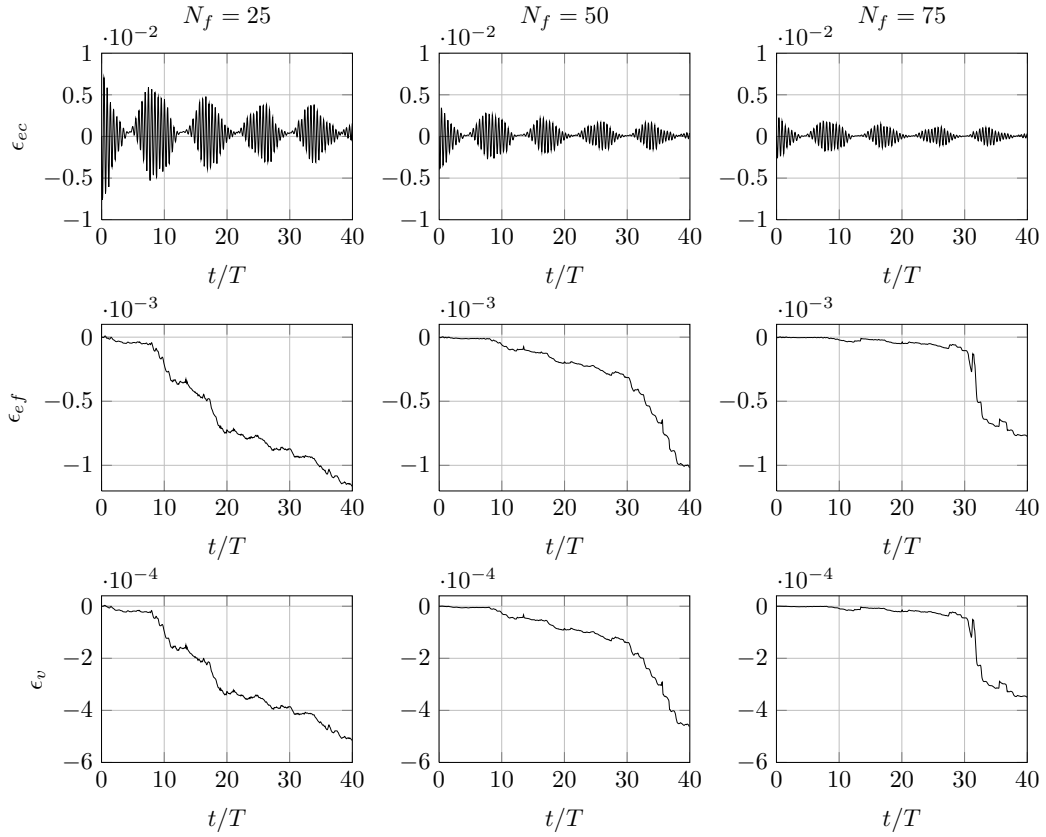
Figure 10: Similar results as Fig. 9, but for the submergence depth z_{eq} = -0.3 m.
