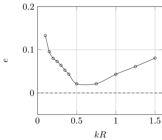
Figure 15: Same case and symbols as in Fig. 14. Computed eccentricity of the trajectory as a function of kR , for H/\lambda = 0.05\% (—o—), compared to Evans et al.'s [27] linear theory (---).
