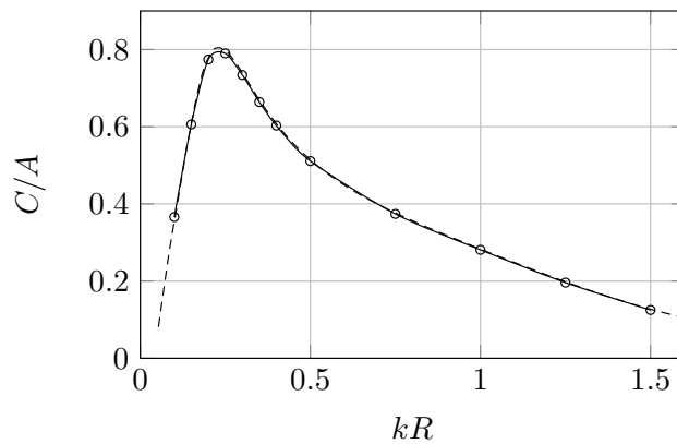
Figure 14: “Bristol cylinder” case. Mean computed radius of the cylinder trajectory as a function of kR , for a wave amplitude H/\lambda = 0.05\% ( -o- ) compared to the prediction of Evans et al.’s [27] linear theory ( - - ).
