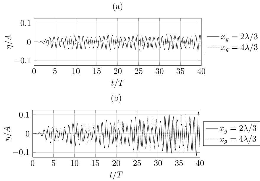
Figure 3: Case of Fig. 2. Non-dimensional free surface elevation (with respect to the amplitude of oscillation A of the cylinder) as a function of non-dimensional time, computed at numerical gages located at x_g = 2\lambda/3 (—) and 4\lambda/3 ( \cdots ) from the cylinder, for two submergence depths z_0 of the cylinder: (a) -0.5 m; (b) -0.4 m. The forced heave amplitude is A = 0.1 m and period T = 0.5 s.
