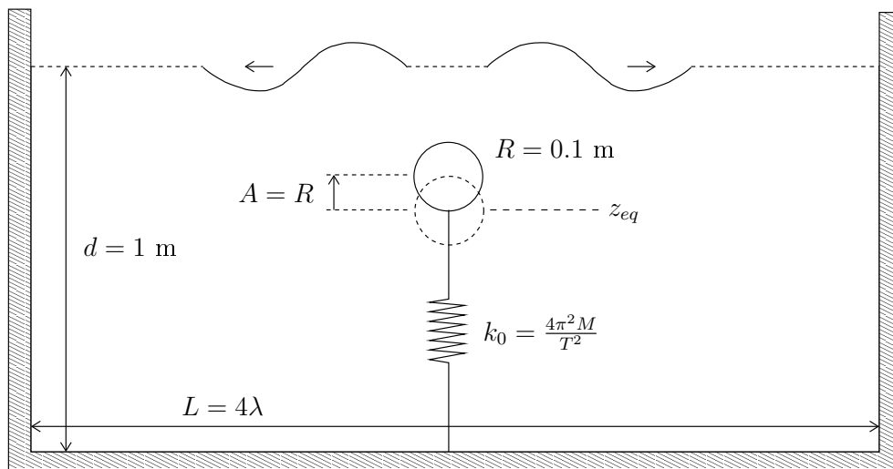
Figure 6: Sketch of problem geometry for a freely heaving cylinder of radius R = 0.1 \text{ m} , following an initial vertical displacement A = R , in water of depth d = 1 \text{ m} . The cylinder is anchored to the bottom of the tank by a spring of stiffness k_0 .
