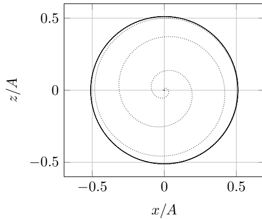
Figure 13: “Bristol cylinder” case for H/\lambda = 0.05\% and kR = 0.51 . Computed location of the cylinder center as a function of time ( \cdots ), compared to the circular path predicted by Evans et al.’s [27] linear theory ( — ).
