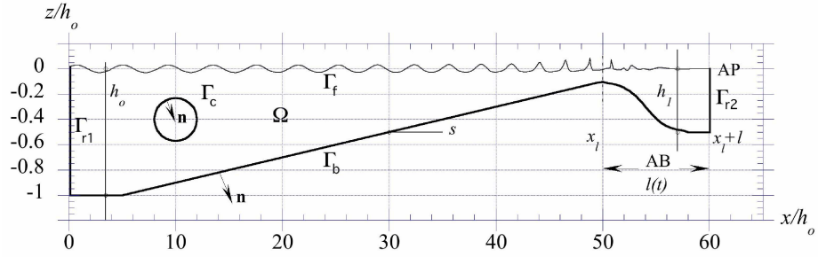
Figure 1: Sketch of computational domain \Omega of 2D-NWT, and its boundaries.
