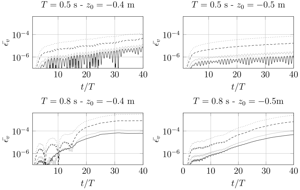
Figure 4: Case of Fig. 2. Error on volume conservation in the computational domain \Omega , for two cylinder submergence depths z_0 and two periods of oscillation T . For each case, results for four spatial free surface discretization steps \Delta x = \lambda/N_f are plotted: N_f = 15 ( \cdots ), N_f = 25 ( --- ), N_f = 50 ( \dots ), N_f = 75 ( --- ).
