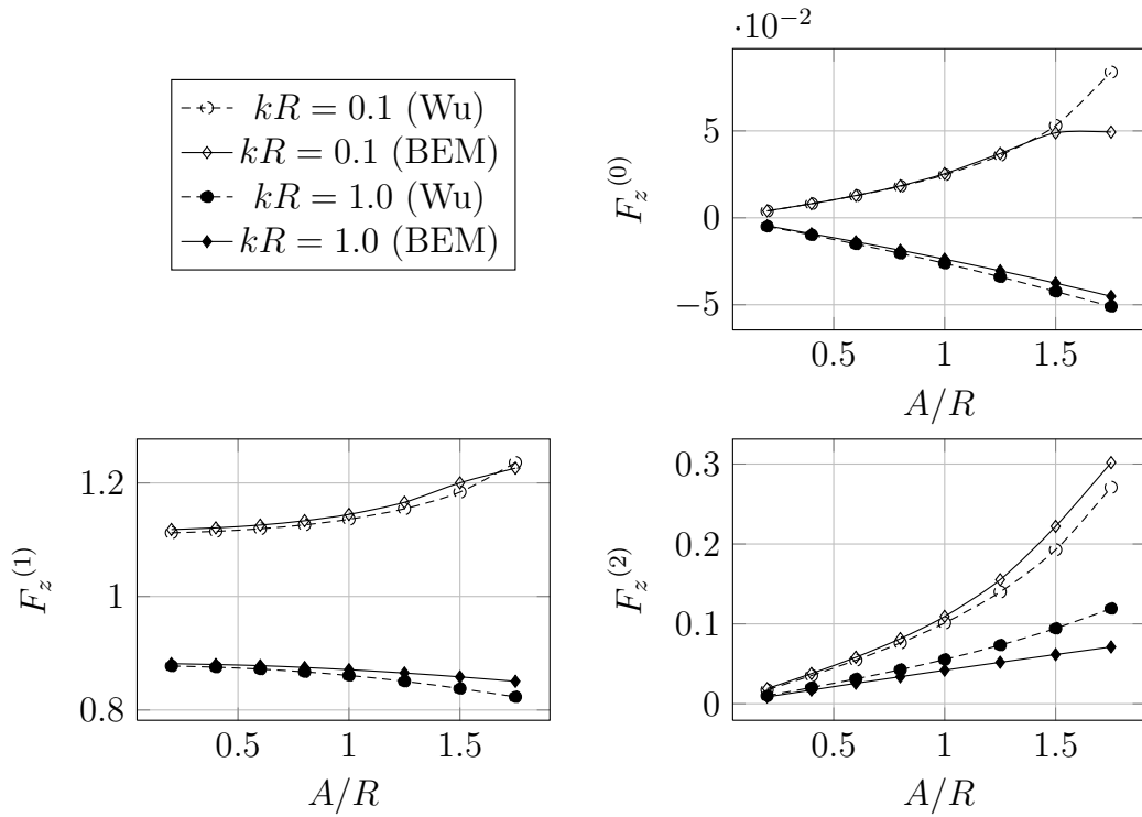
Figure 12: Case of Fig. 11. Nondimensional 0 th -order (mean), 1 st and 2 nd harmonics of the vertical force. BEM/NWT results compared to Wu's semi-linear theory for various amplitudes of body motion A/R and for two frequencies of oscillation ( kR = 0.1 and kR = 1 ).
