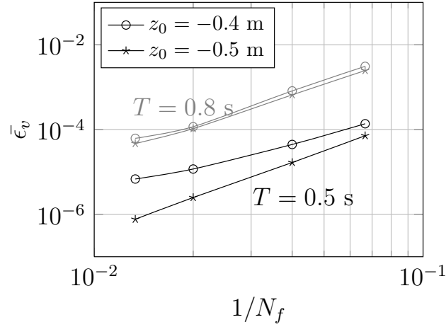
Figure 5: Case of Fig. 2. Mean volume error after 40 periods of heave oscillation, for T = 0.5 s and T = 0.8 s and two cylinder submergence depths, as a function of the nondimensional discretization step 1/N_f = \Delta x/\lambda .
