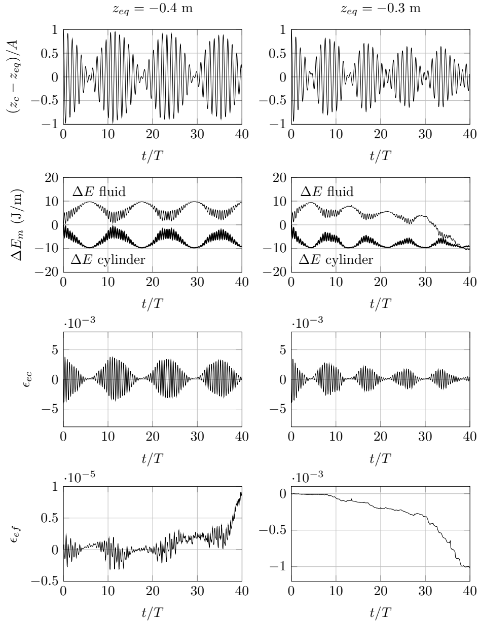
Figure 7: Time series of nondimensional vertical position of the cylinder from equilibrium depth (upper row), the fluid and cylinder mechanical energy variations from initial instant (second row), the relative error in the cylinder energy conservation (third row) and the relative error in fluid energy conservation (lower row), as a function of nondimensional time t/T . In the BEM, 60 nodes are used on the cylinder boundary and N_f = 50 nodes per wavelength on the free surface. Results for the case on Fig. 6, for submergence depth z_{eq} = -0.4 m (left column) and z_{eq} = -0.3 m (right column)
