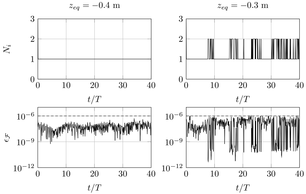
Figure 8: Time series of the number N_i of sub-iterations required to achieve convergence of the body hydrodynamic pressure force (upper row), and relative error \epsilon_{\mathcal{F}} on the latter at convergence (lower row); the 10^{-6} convergence threshold is marked on the figure (- -). Results for the case on Fig. 6, for submergence depth z_{eq} = -0.4 m (left column) and z_{eq} = -0.3 m (right column).
