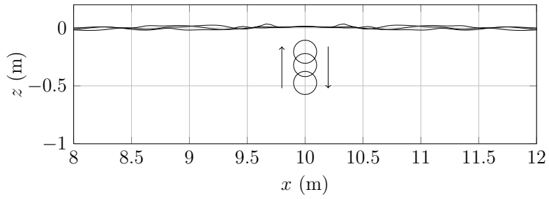
Figure 11: Forced heaving motion of a cylinder of radius R = 0.1 m in depth d = 3 m. Successive snapshots of waves generated at t/T = 2.75, 2.99, 3.10 for an amplitude A/R = 1.75 , and kR = 0.1 (period T = 2.01 s).
