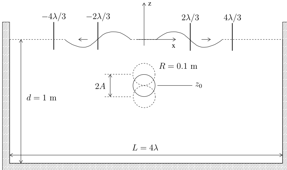
Figure 2: Sketch of problem geometry for a cylinder of radius R = 0.1 m in forced heaving motion of amplitude A = R and period T , in water of depth d = 1 m.
