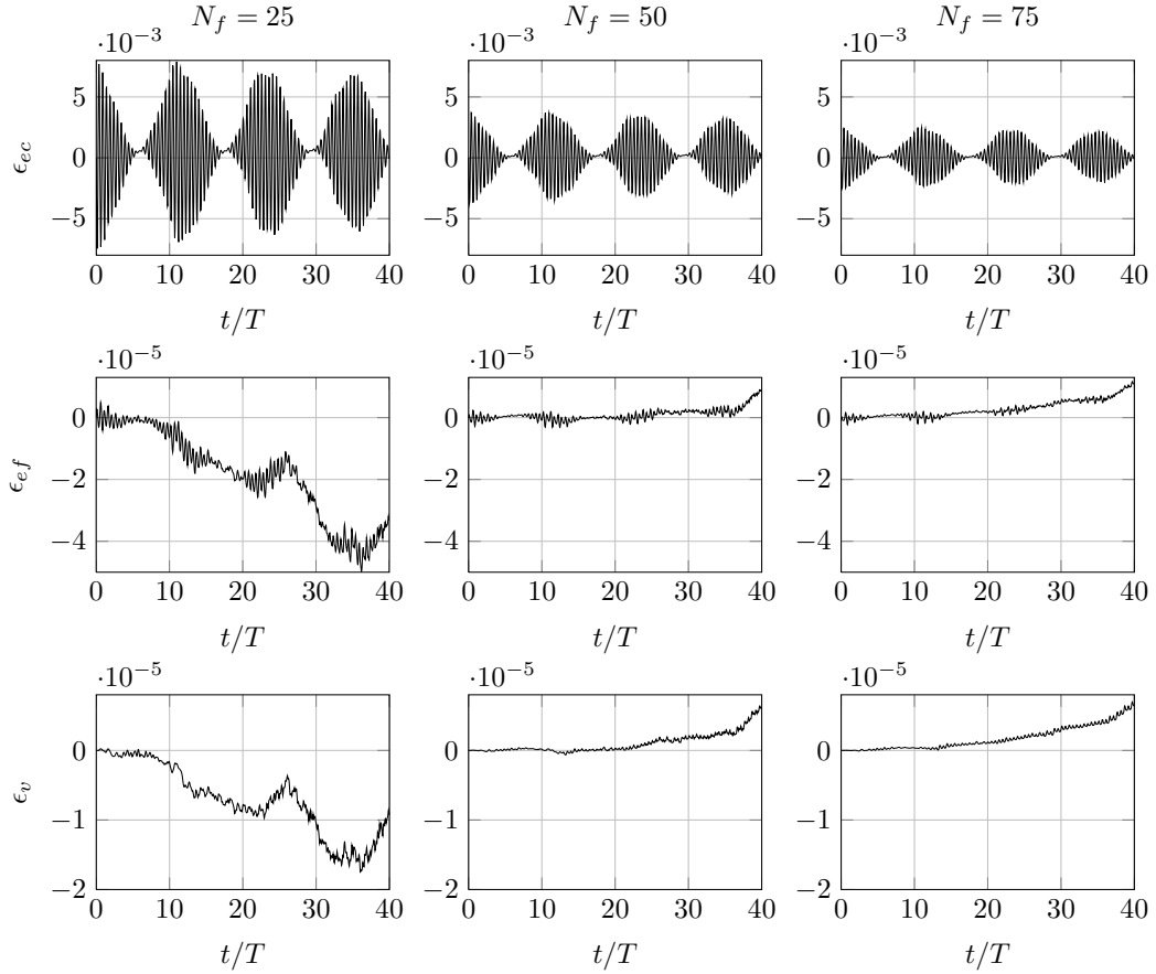
Figure 9: From top to bottom, time series of cylinder energy error, fluid energy error and fluid volume conservation error. In each column are shown the numerical relative errors for three spatial discretization steps on the free surface boundary: N_f = 25 (left column), N_f = 50 (central column), N_f = 75 (right column). Results for the case on Fig. 6, for submergence depth z_{eq} = -0.4 m.
