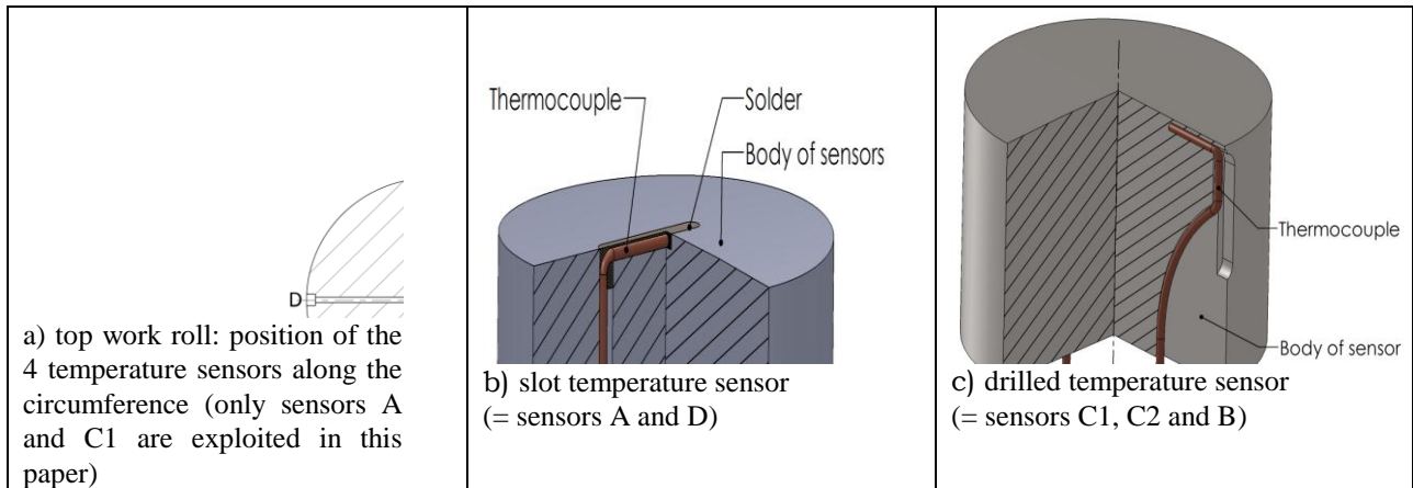
Fig. 1: temperature sensors
