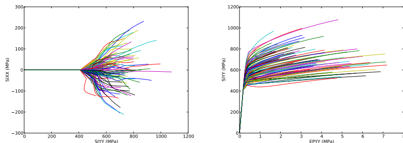
Fig. 6 Mesoscopic behavior in each grain in the X (left) and Y (right) directions
