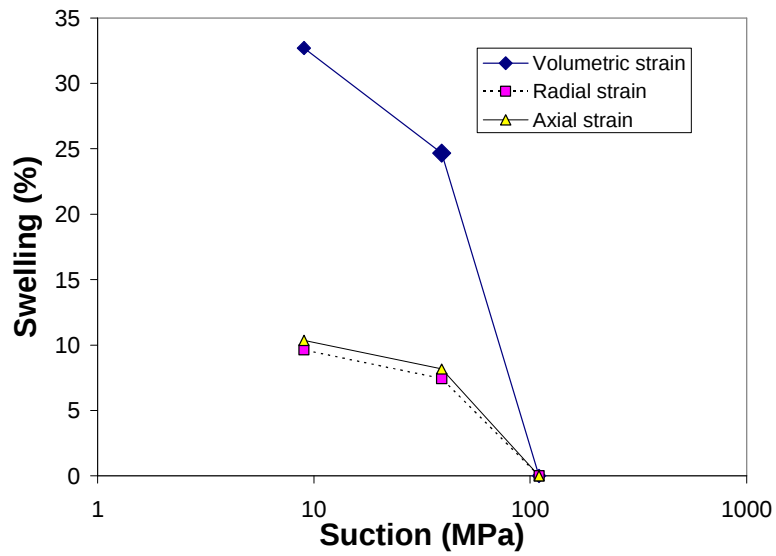
Fig. 5. Axial, radial and volumetric strain during wetting
