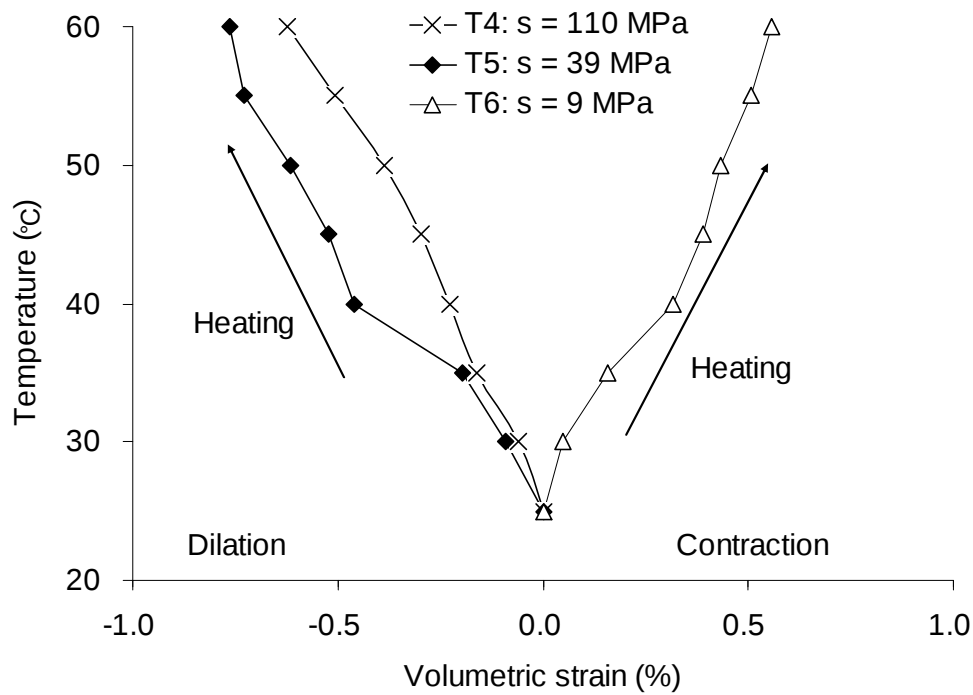
Fig. 6. Volumetric strain during thermal loading under constant pressure at 0.1 MPa: tests T4-T6
