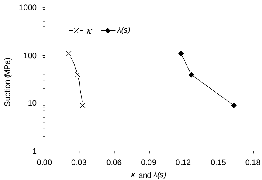
Fig. 8. Compressibility parameters \kappa and \lambda(s) versus suction for tests at 25 °C
