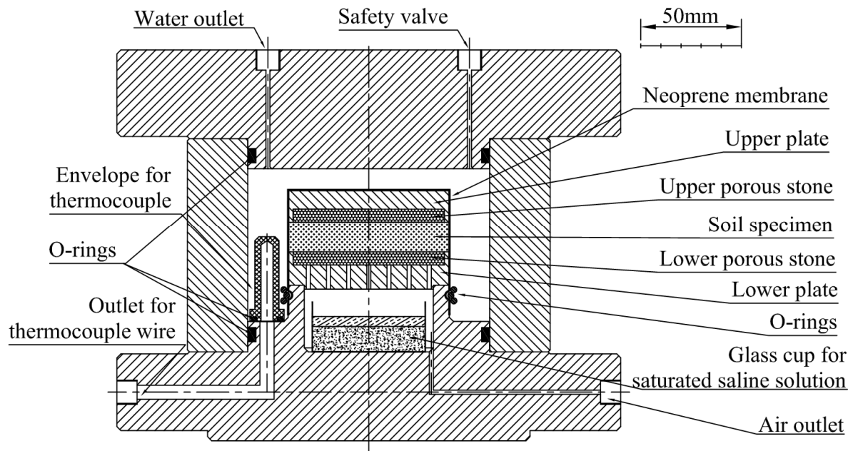
Fig. 1. Basic scheme of the suction-temperature controlled isotropic cell (after Tang et al., 2007)
