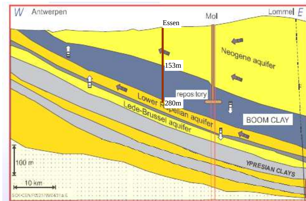
Figure 3. Hydrogeological cross-section (Wemaere et al. , 2008)
