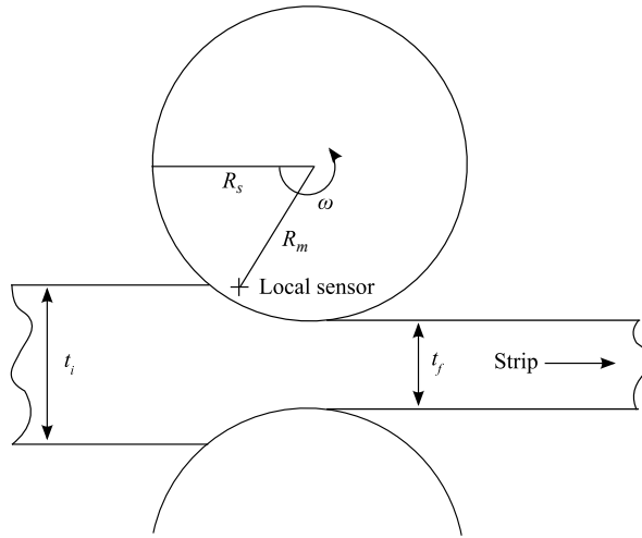
Figure 1: Rolling process
