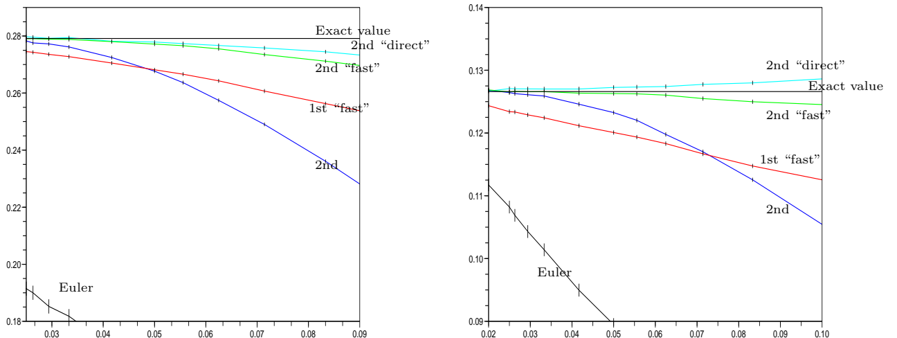
Figure 1: d = 3 , same parameters as for Table 1. In the left (resp. right) side is plotted (50) (resp. \mathbb{E} \left[ \sum_{1 \leq i \neq j \leq d} (\hat{X}_T^N)_{i,j} \right] ) in function of the time step 1/N . The width of each point represents the 95% confidence interval ( 10^7 scenarios for the modified Euler scheme and 10^8 for the others).
