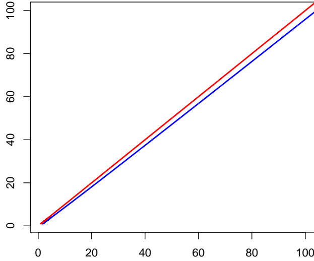
FIG 3. The curve of the function L \rightarrow \gamma_L (blue) and the bissectrice (red).
