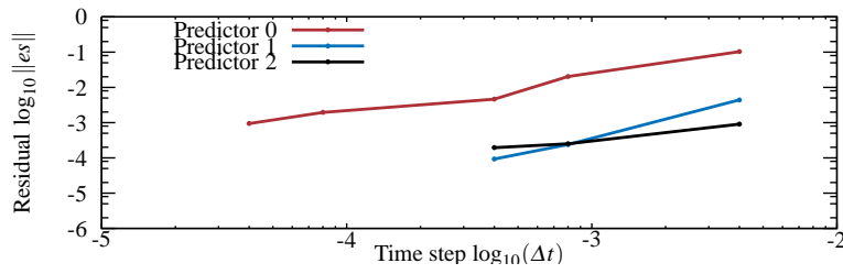
Fig. 20 Maximum residual error for explicit coupling schemes with different time step sizes and predictors.
