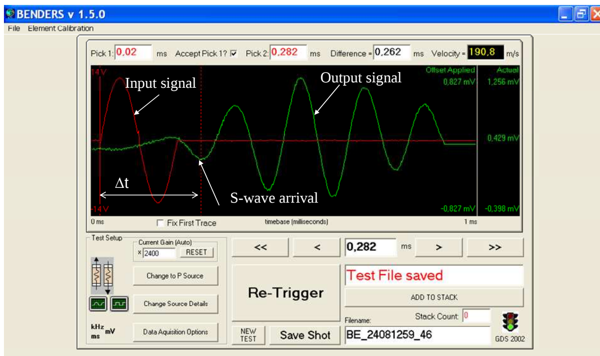
Figure 4. Response of shear wave for the soil sample treated with 3% of lime, D_{max} = 5 mm, w_i = 14\% , 886 h after the treatment
